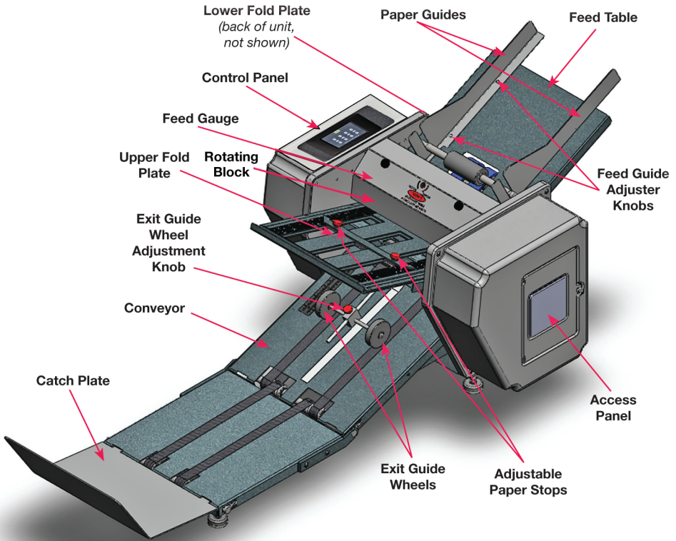
Figure 6: Machine Diagram
