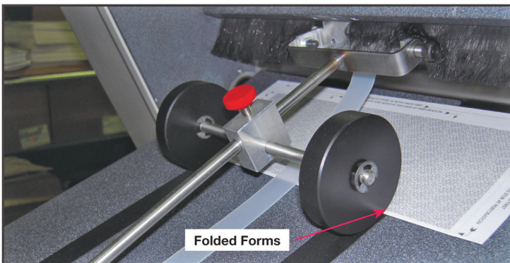
Figure 12: Exit Guide Wheel Adjustment
